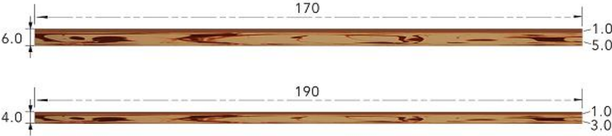
Side View
